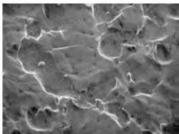
Scanning electron micrograph of an Extragal ® coating surface.
